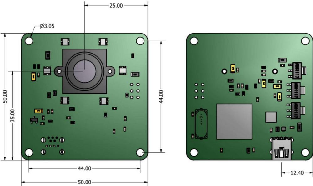
Figure 1 Dimensional drawing of I3-C202 module
