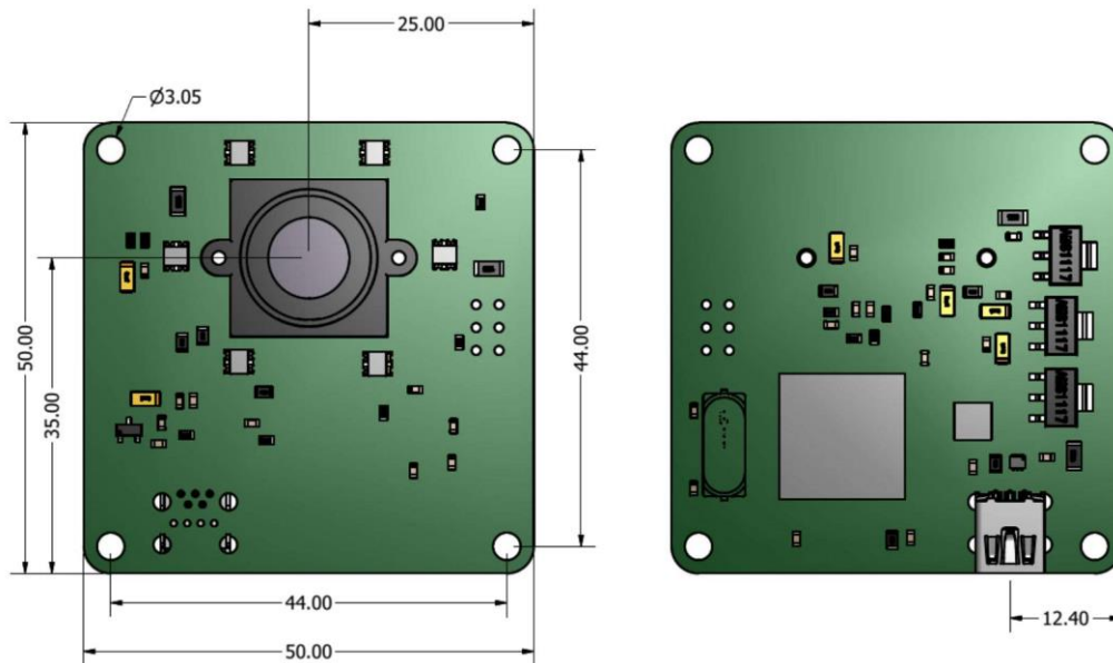
Figure 1 Dimensional drawing of I3-C201
